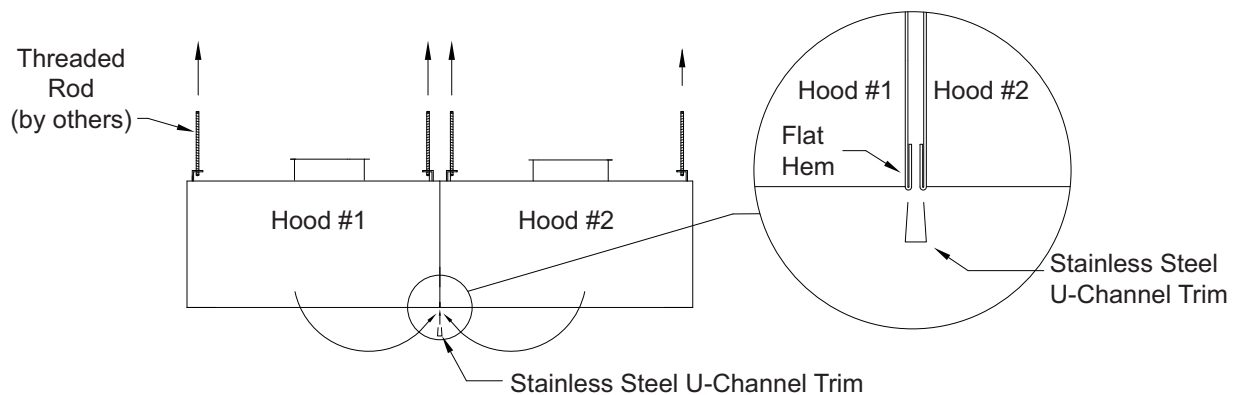
Figure 12 - Back-to-Back Hoods
